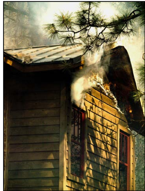
Figure 4.13. Firefighters must evaluate ember traps such as gable end and foundation vents, where embers can enter and ignite a structure. Photo courtesy of Kari Greer.
